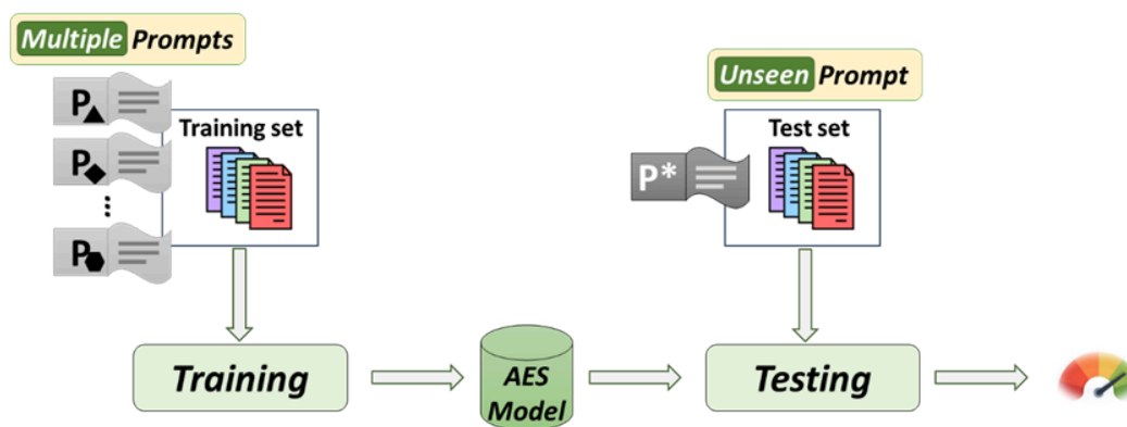
Figure 4. Learning a Cross-prompt AES model.
